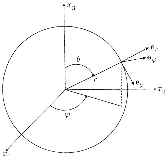
FIGURE 1. Spherical coordinates
